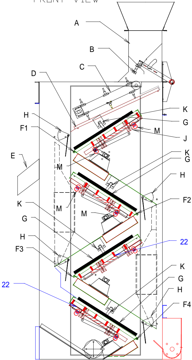
FRONT VIEW
